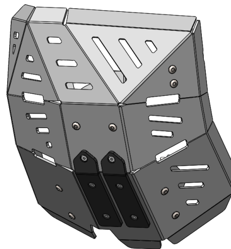
ALUMINUM TRAIL ENGINE GUARD Ref.: 2CP0900083
