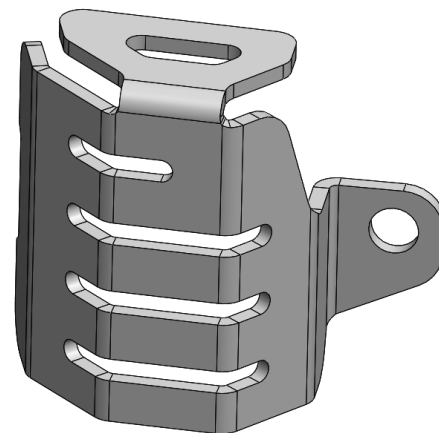
REAR BRAKE FLUID RESERVOIR GUARD Ref.: 2CP2180087
