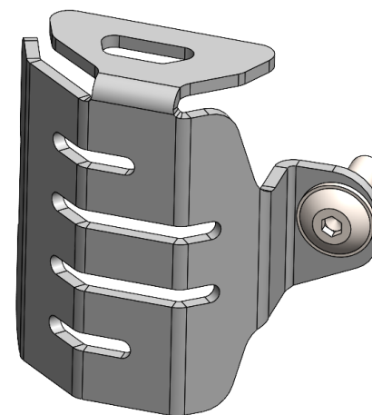
REAR BRAKE FLUID RESERVOIR GUARD Ref.: 2CP2180090
